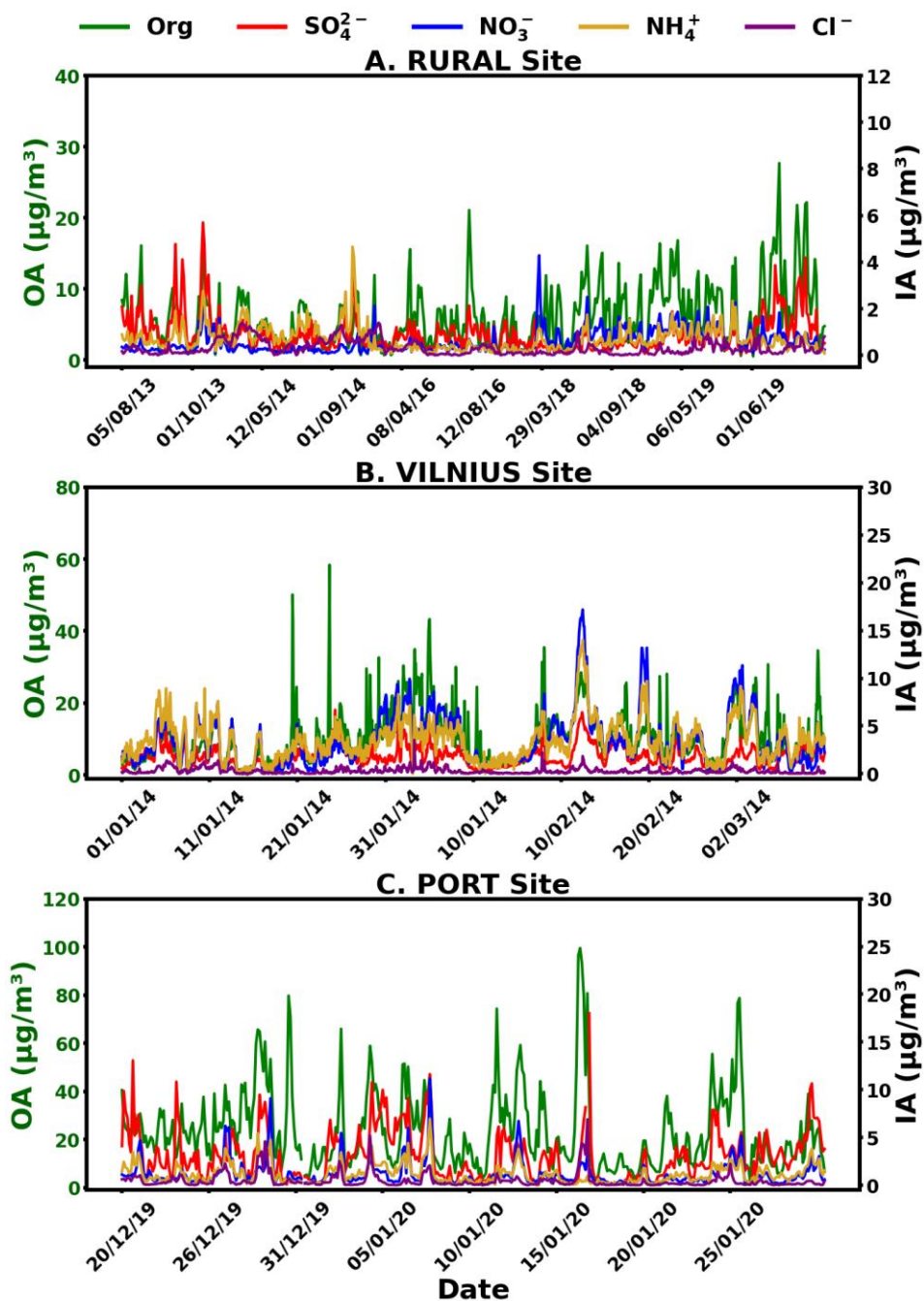
Fig. 5. The hourly average time series of OA, \text{SO}_4^{2-} , \text{NO}_3^- , \text{NH}_4^+ , and \text{Cl}^- at Rūgštelėškis rural site (Lithuania) (A), Vilnius city site (Lithuania) (B), and Manila port site (Philippines) (C).
