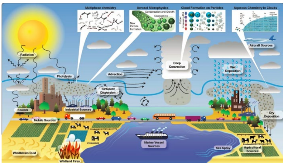
Figure 2. The different sources of \text{PM}_{2.5} in the environment (source: https://www.epa.gov/cmaq/overview-science-processes-cmaq )
