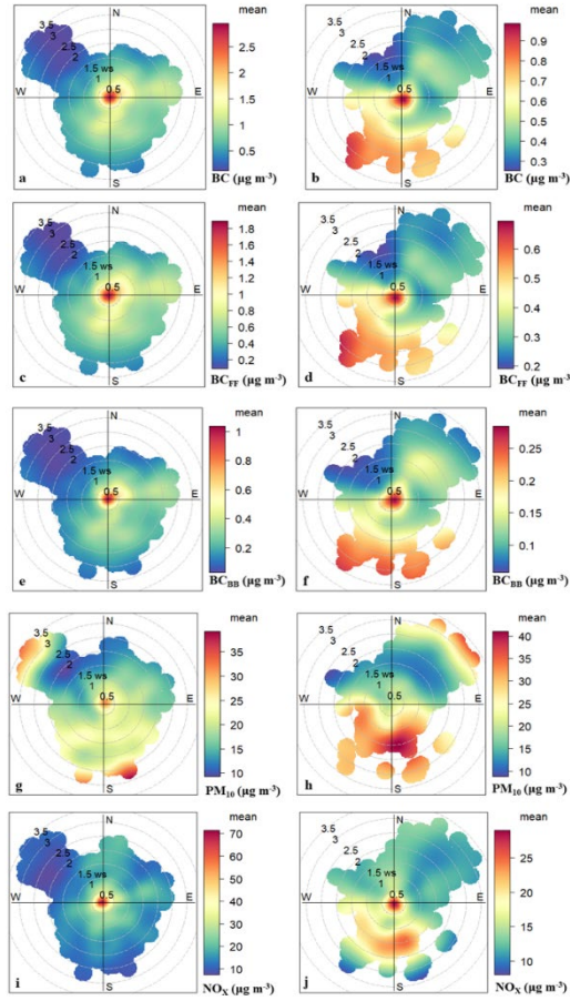
Figure 17. Polar plots of BC, BC FF , BC BB , PM 10 and NO x mass concentration as a function of wind speed and direction for heating (a, c, e, g, i) and non-heating season periods (b, d, f, h, j).
