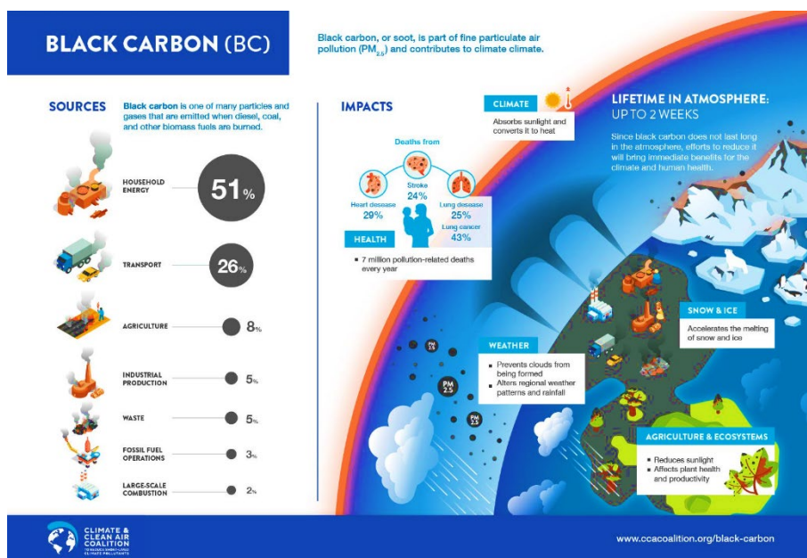
Figure 4. Source breakdown and impact overview of BC from the climate and clean air coalition (Climate & Clean Air Coalition 2018).
