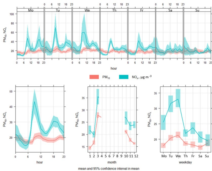
Figure 13. Time variation plots to show the mean pollutant concentrations with respect to their averaging times for PM_{10} and NO_x by hour of weekday, by hour, by month and by weekday for the heating season period.
