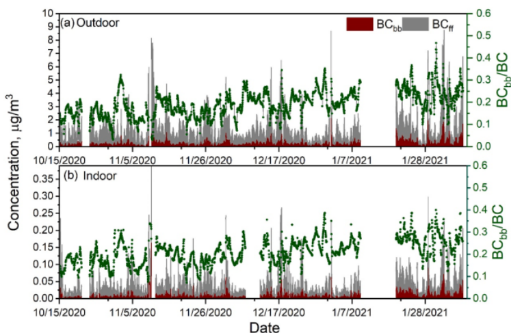
Figure 32. \text{BC}_{\text{FF}} and \text{BC}_{\text{BB}} concentration and \text{BC}_{\text{BB}}/\text{BC} ratios in outdoor (a) and indoor (b) samples.
