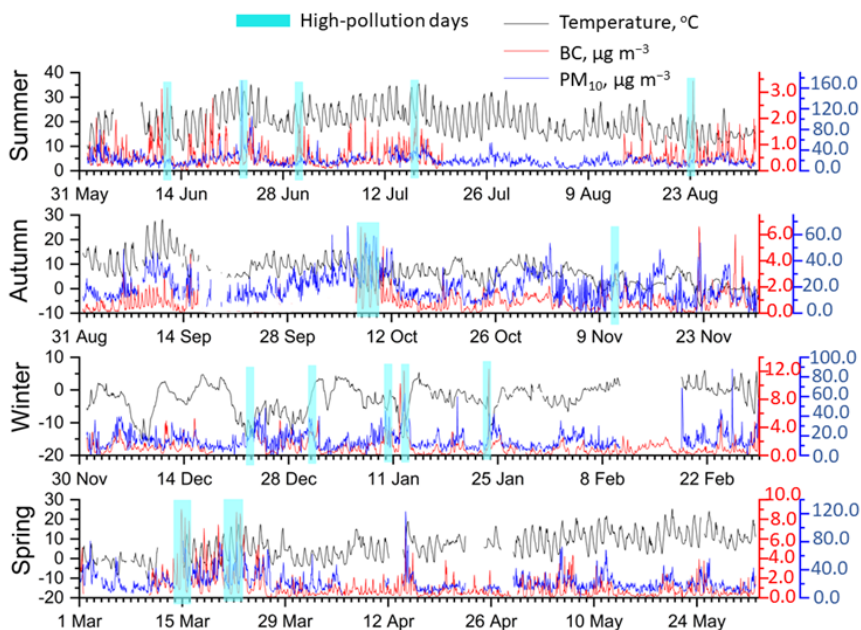
Figure 27. The time series of BC, PM 10 and air temperature during the four seasons with pronounced days of high air pollution (blue rectangles—periods with hourly BC mass concentration exceeding the 95 th percentile of the BC concentration for the respective season).
