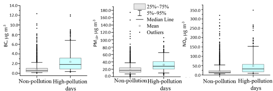
Figure 28. The comparison of BC, PM 10 and NO x concentrations on non-pollution and high-pollution days.
